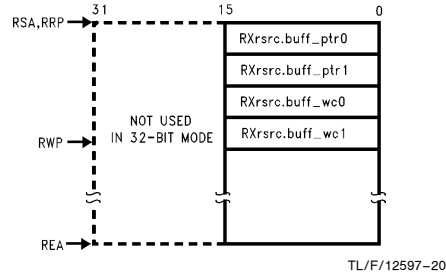
FIGURE 5-9. RRA Initialization
